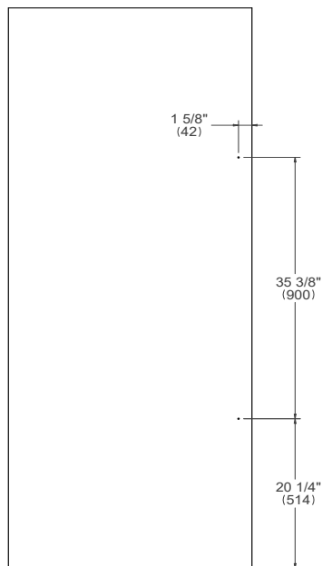
BERTAZZONI HANDLES DRILLING ON LEFT SWING REFRIGERATOR DOOR
