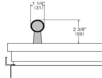
BERTAZZONI HANDLES DRILLING ON RIGHT SWING REFRIGERATOR DOOR
