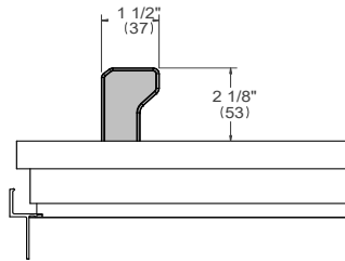
BERTAZZONI HANDLES DRILLING ON LEFT SWING REFRIGERATOR DOOR
