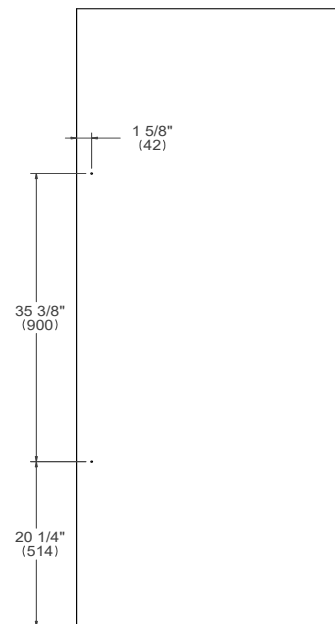
BERTAZZONI HANDLES DRILLING ON RIGHT SWING REFRIGERATOR DOOR
