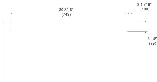
BERTAZZONI HANDLES 36" (90CM) FREEZER DRAWER
